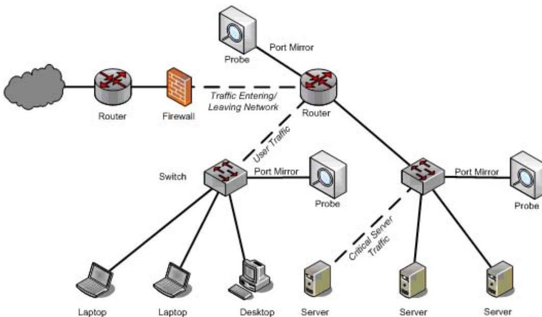
Figure 2 - Probe Deployment using Port Mirrors
