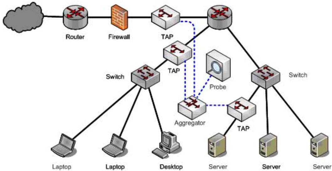
Figure 4 - Aggregation of TAP Outputs to a single Probe
