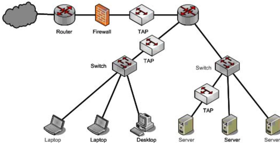
Figure 3 – Common Network TAP Locations
